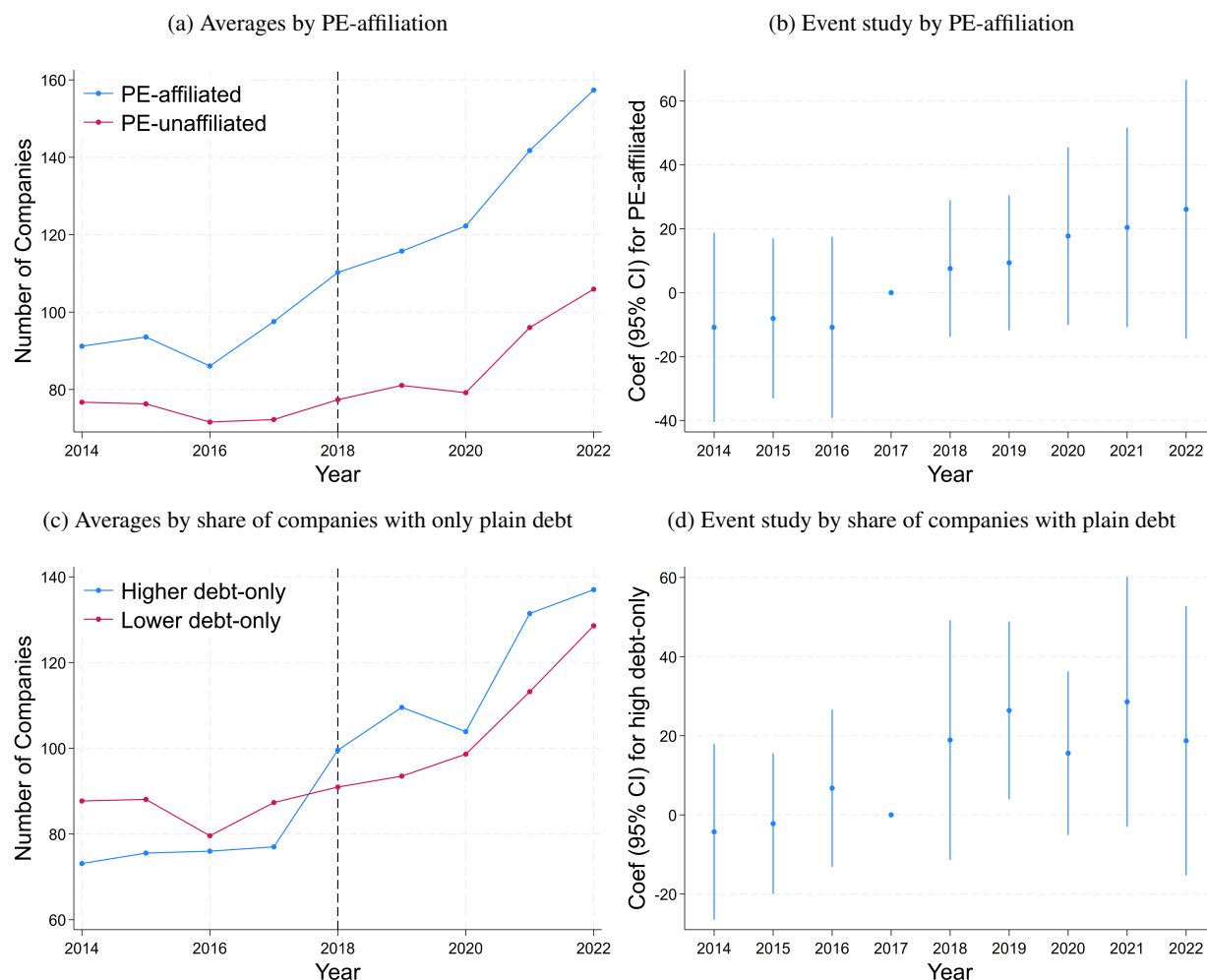
Figure A.6: Event study analysis: Number of BDC-company relationships
