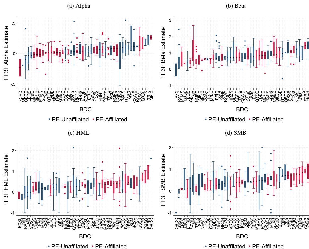
Figure A.5: Fama-French Three-Factor Model estimates: Within- and between-BDC variation
