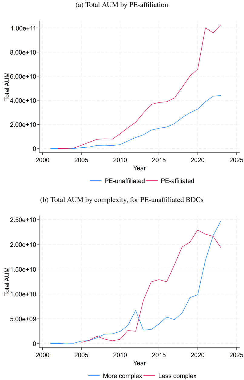
Figure 8: Decomposing the growth of BDCs
